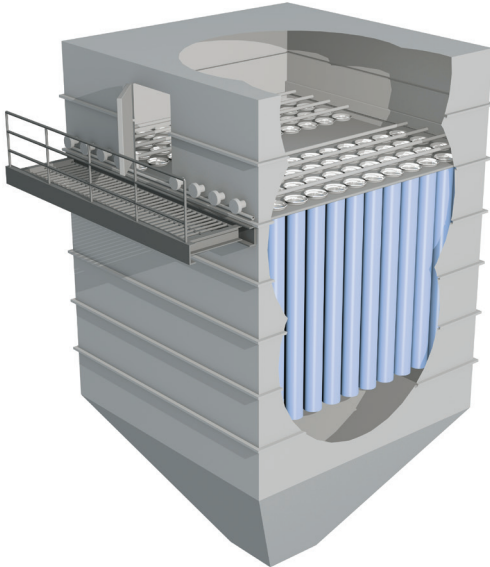
Pulse-Jet Systems
